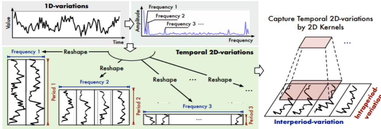
Figure 2: A univariate example to illustrate 2D structure in time series. By discovering the periodicity, we can transform the original 1D time series into structured 2D tensors, which can be processed by 2D kernels conveniently. By conducting the same reshape operation to all variates of time series, we can extend the above process to multivariate time series.
